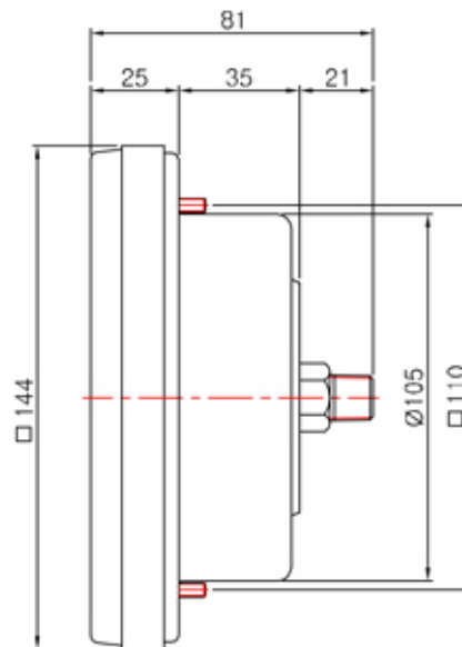
Male PT 1/4"
